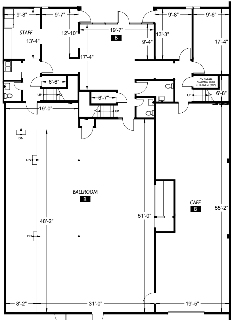
FLOOR 1
