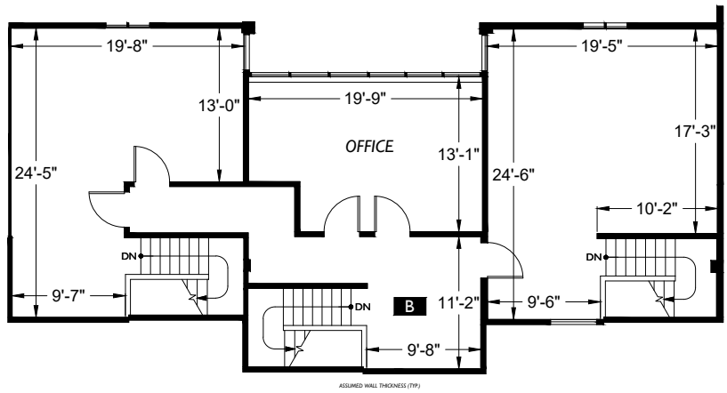
FLOOR 2
