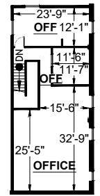
MEZZANINE
