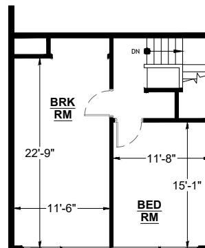
MEZZANINE
