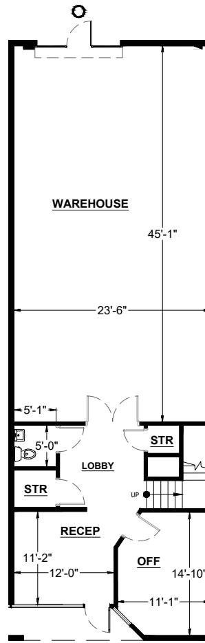
GROUND LEVEL
